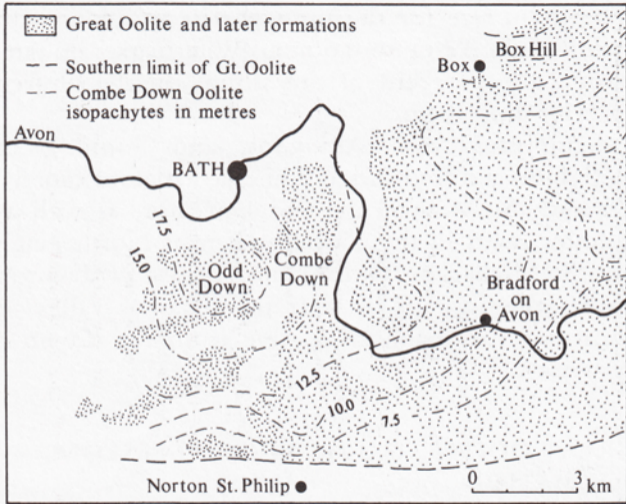
FIGURE 6 Isopachytes of the Combe Down Oolite
